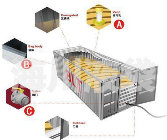
STRUCTURE OF FLEXITANK
